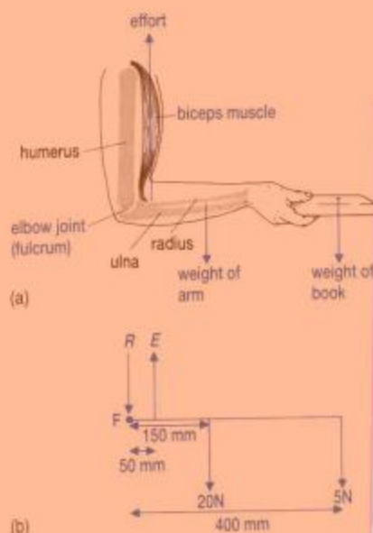
FIG 1.4 The lower arm as a lever.
