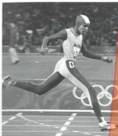
FIG 1.12 Kathy Freeman conserves angular momentum while running in the Olympic Games.
