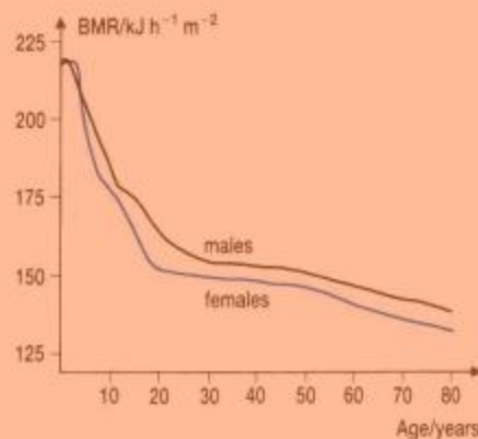
FIG 1.15 Basal metabolic rate variation with age and sex.
